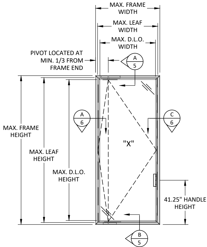
"X" ELEVATION TYPICAL
