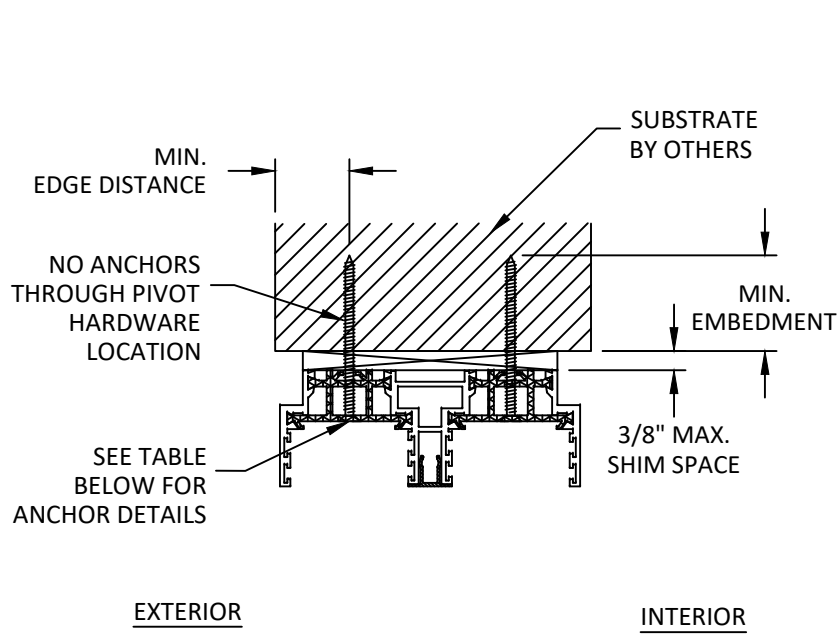
A 7 VERTICAL SECTION HEAD - THROUGH FRAME
