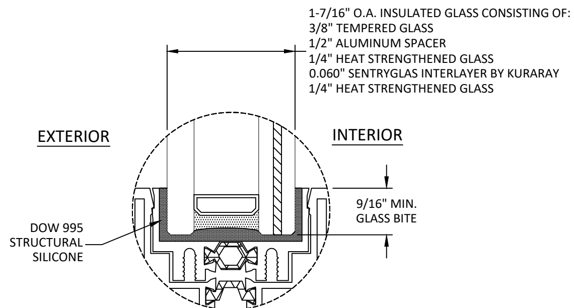
GLAZING DETAIL 1
