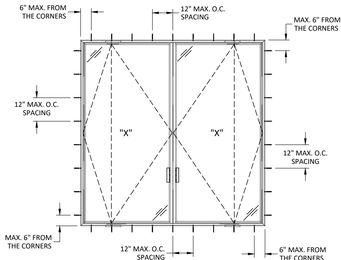
"XX" ANCHOR LAYOUT
