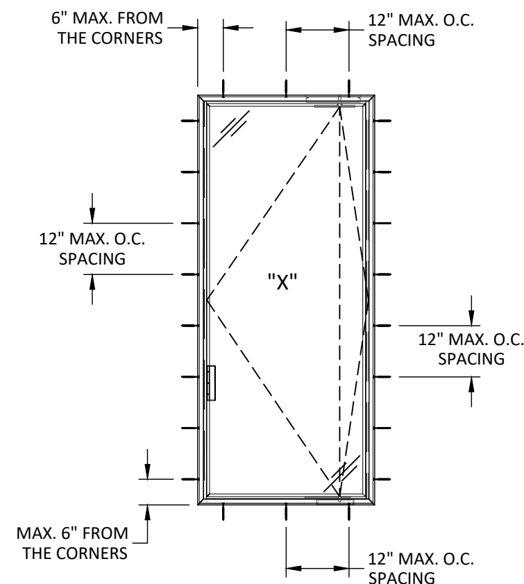
"X" ANCHOR LAYOUT THROUGH FRAME INSTALLATION
