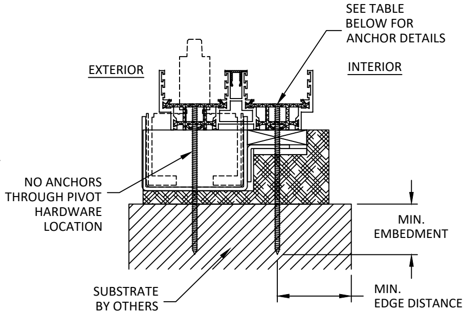
B 7 VERTICAL SECTION SILL - THROUGH FRAME
